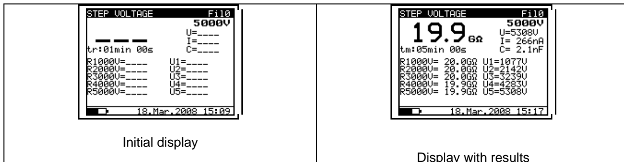
Fig. 22. Step Voltage function display states- Graph R(t) disabled
