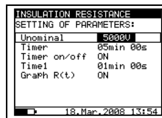
Fig. 13. Set-up menu in Insulation Resistance measurement
