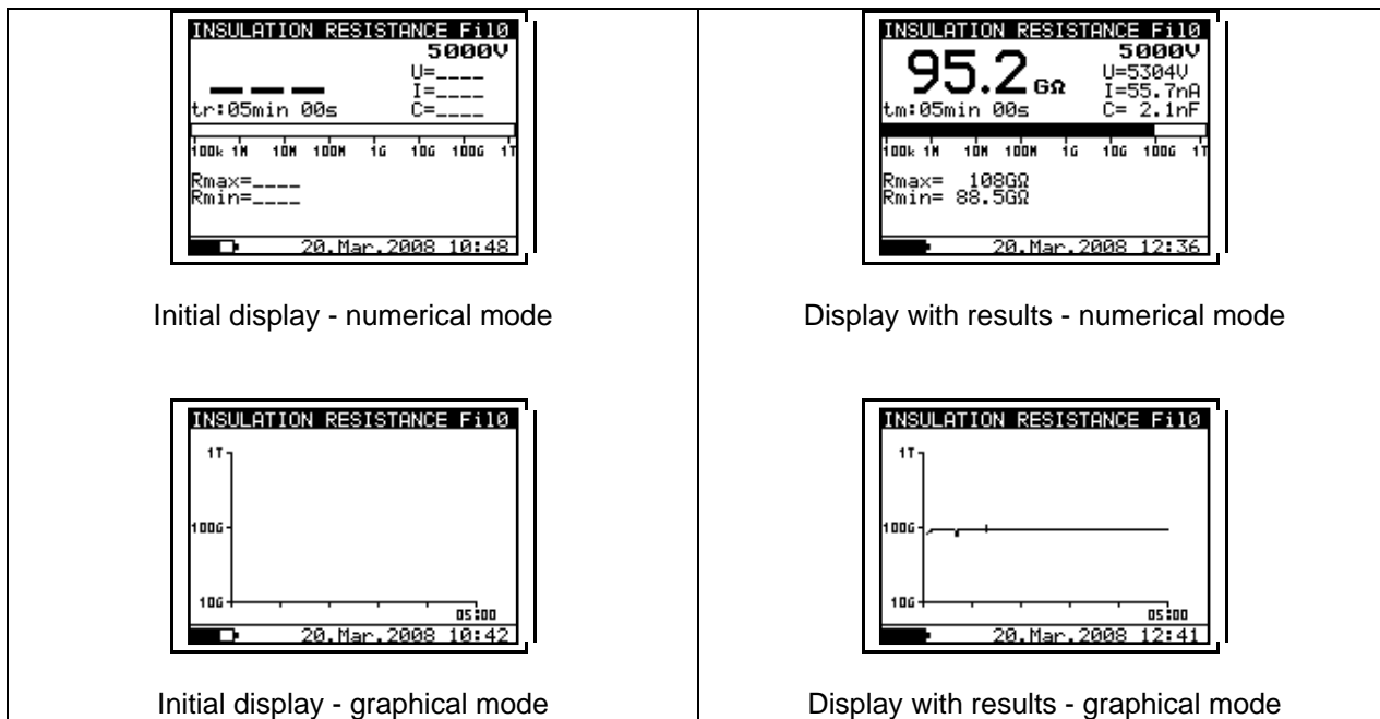
Fig. 12. Insulation Resistance function display states - Graph R(t) enabled
