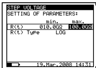
Fig. 27. Set-up menu of the Graph R(t)
