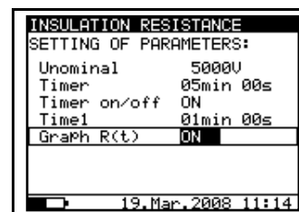
Fig. 14. Set-up menu in Insulation Resistance measurement
