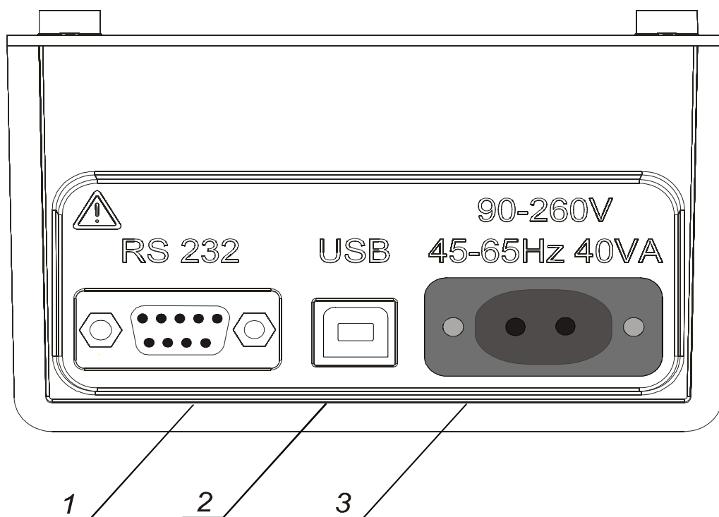
Fig. 3. Communication and Mains connector
