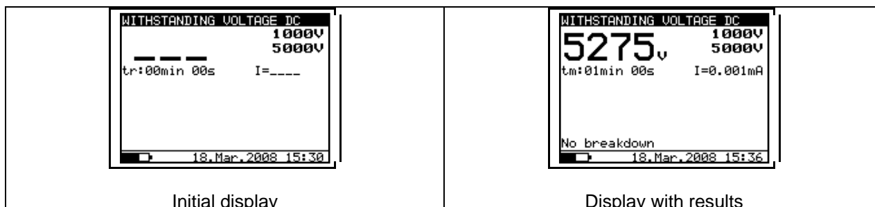
Fig. 29. Withstanding Voltage function display states
