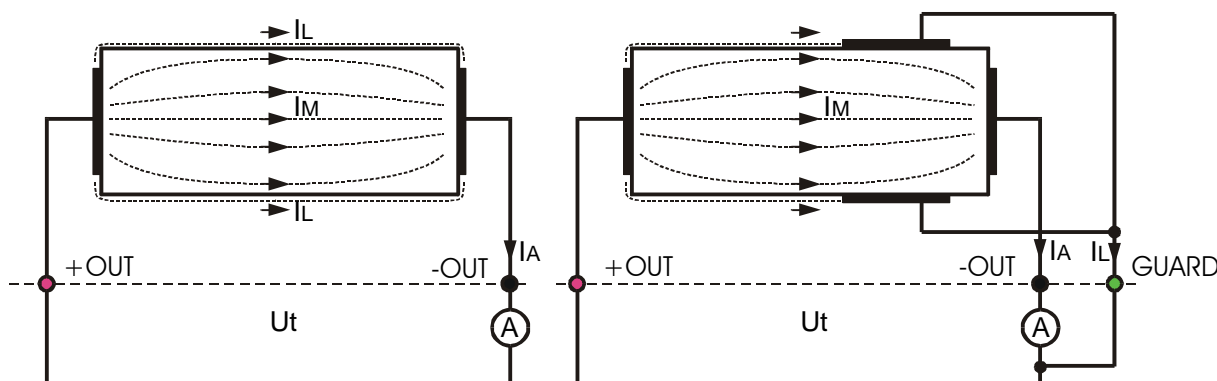
Fig. 9. Connection of GUARD terminal to measured object
