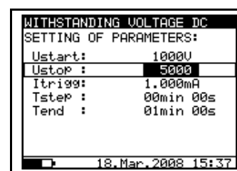
Fig. 30. Set-up menu in Withstanding Voltage function
