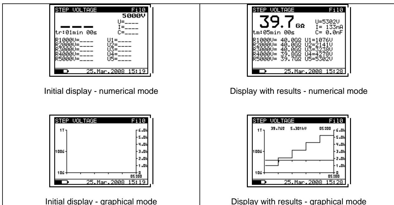
Fig. 23. Step Voltage function display states - Graph R(t) enabled
