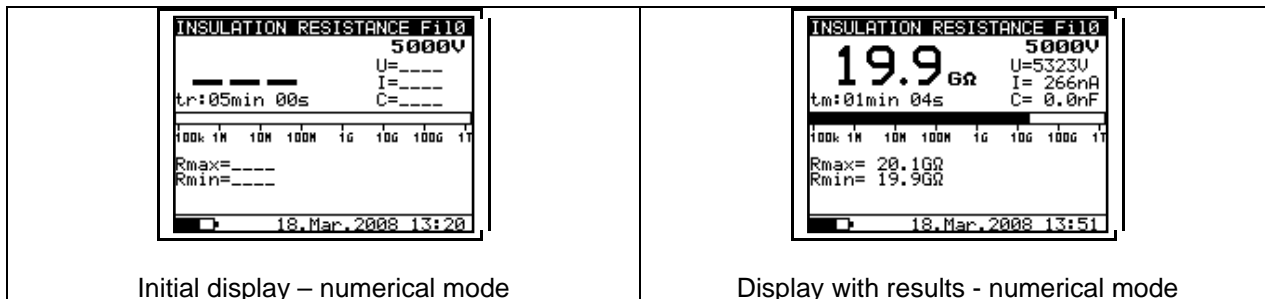
Fig. 11. Insulation Resistance function display states - Graph R(t) disabled
