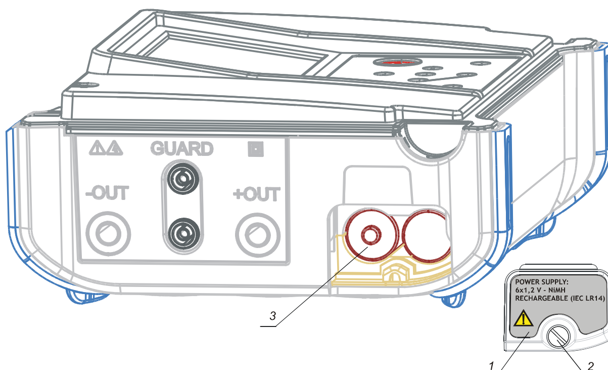
Fig. 32. Correct polarity of inserted batteries
