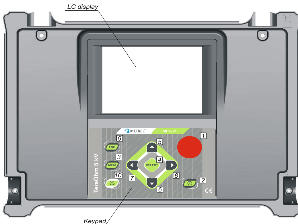
Fig. 1. Front panel
