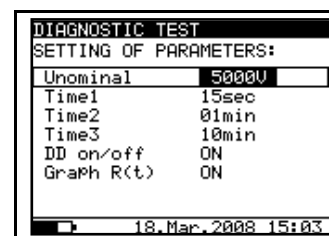
Fig. 18. Set-up menu in Diagnostic Test
