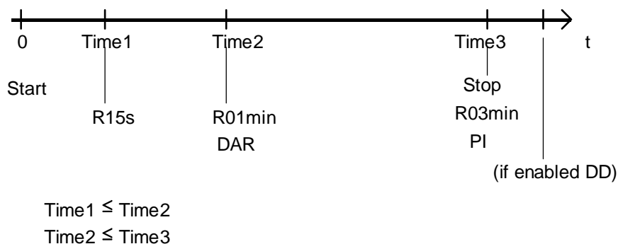
Fig. 19. Timer relations
