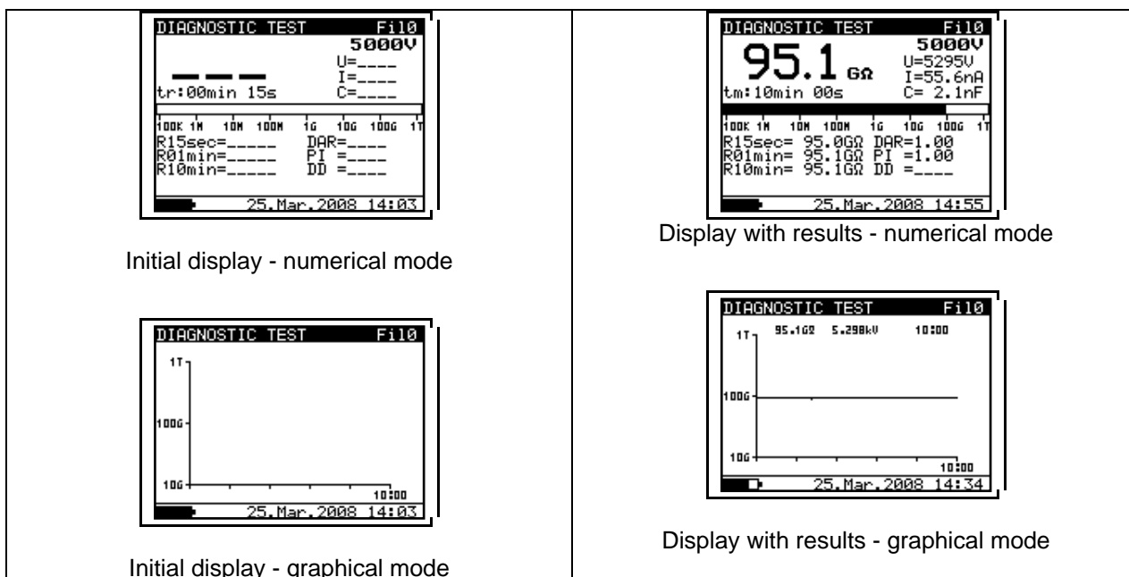
Fig. 17. Diagnostic test display states - Graph R(t) enabled
